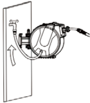
Connect the side connector to the tap
